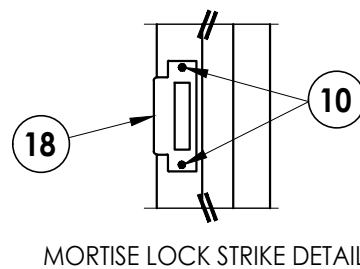
LATCH & DEADBOLT STRIKE DETAIL
